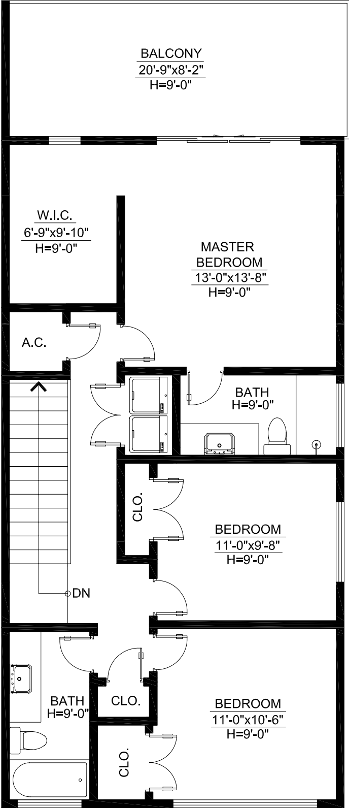
UPPER FLOOR PLAN FLOOR AREA: 898 sq.ft.
