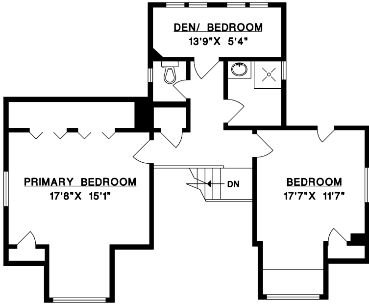
UPPER FLOOR
